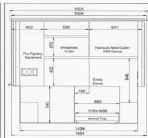
Figure 2: Cabinet-Storage Based Route Patrolling Vehicle Arrangement
