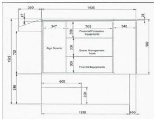
Figure 2: Cabinet-Storage Based Route Patrolling Vehicle Arrangement
