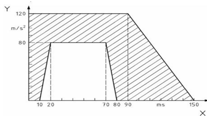
Fig. 2 Acceleration Impulse
